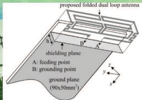
Antenna for Mobile Handset Applications
