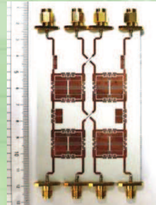
Miniaturized BUTLER MATRIX Network for BEAMFORMING-SWITCHED Array
