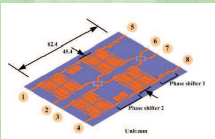
Miniaturized BUTLER MATRIX Network for BEAMFORMING-SWITCHED Array
