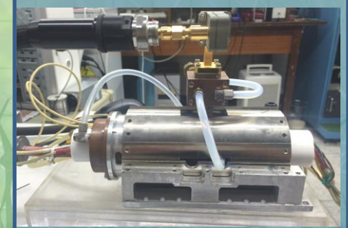
Microwave Source
