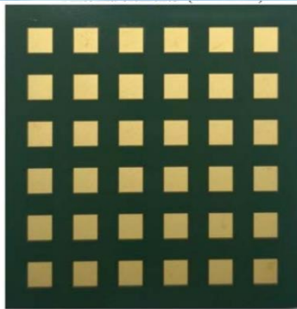
5G FR2 Antenna in Package
