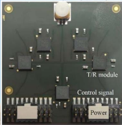
5G FR2 Antenna in Package
