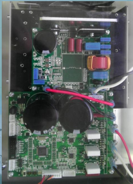
AC/DC/AC Power Converter
